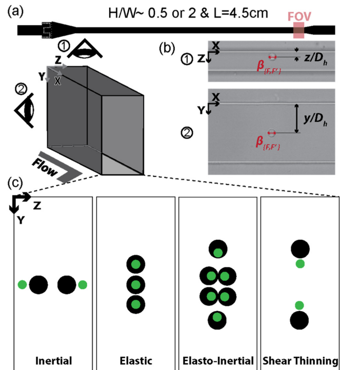
FIG. 1. Experiment design overview: (a) the schematic depicting the experimental setup. (b) High-speed microscopic images of hydrodynamically focused MIN6 cells in the microchannels with the cross-section of high and low aspect ratios. The high-speed videos were captured at the field of view (FOV) located at 4.5 cm from the inlet. The annotations indicate the dimensionless lateral focusing positions of cells \frac{y}{D_h} and \frac{z}{D_h} and the blockage ratios, \beta . (c) The schematics illustrate the cross-sectional cell focusing arrangements under the tested various flow conditions, namely, inertial, elastic dominant, elasto-inertial, and elasto-inertial with strong shear thinning.
